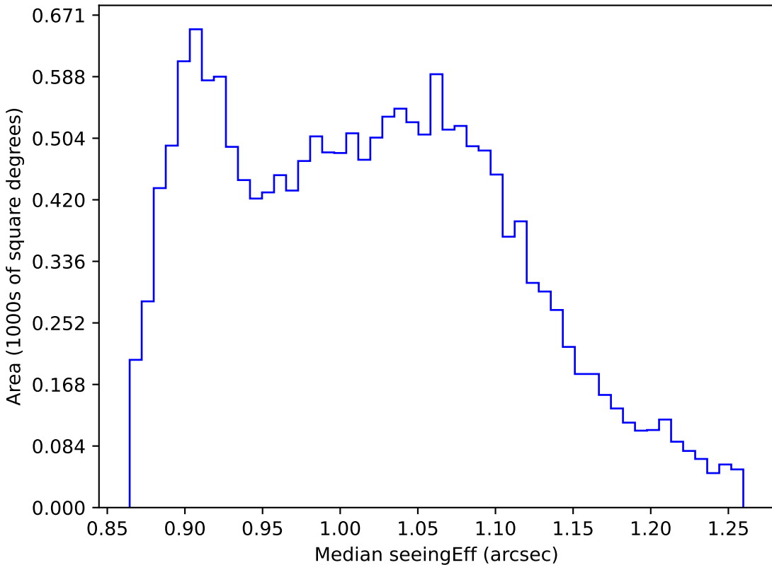
noroll_mjdp180_v3.4_10yrs WFD r band: Median seeingEff
