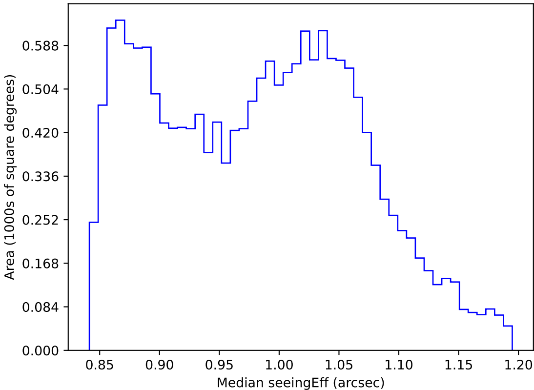
noroll_mjdp180_v3.4_10yrs WFD i band: Median seeingEff
