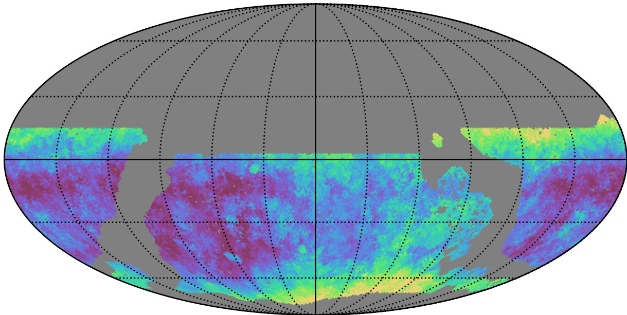
noroll_mjdp180_v3.4_10yrs WFD g band: Median seeingEff
