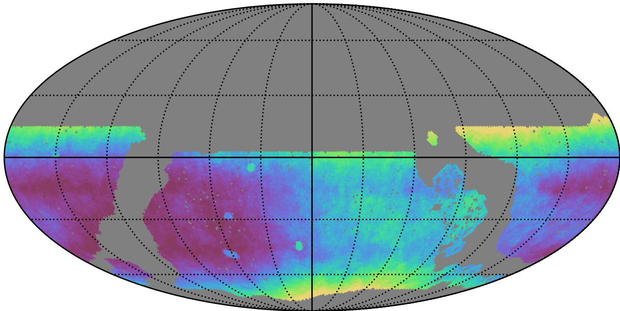
noroll_mjdp180_v3.4_10yrs WFD all bands: Median seeingEff
