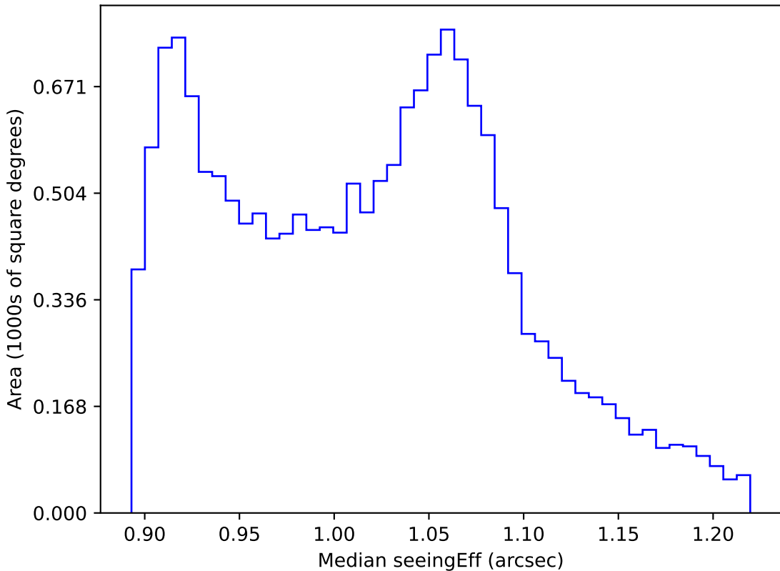
noroll_mjdp180_v3.4_10yrs WFD all bands: Median seeingEff
