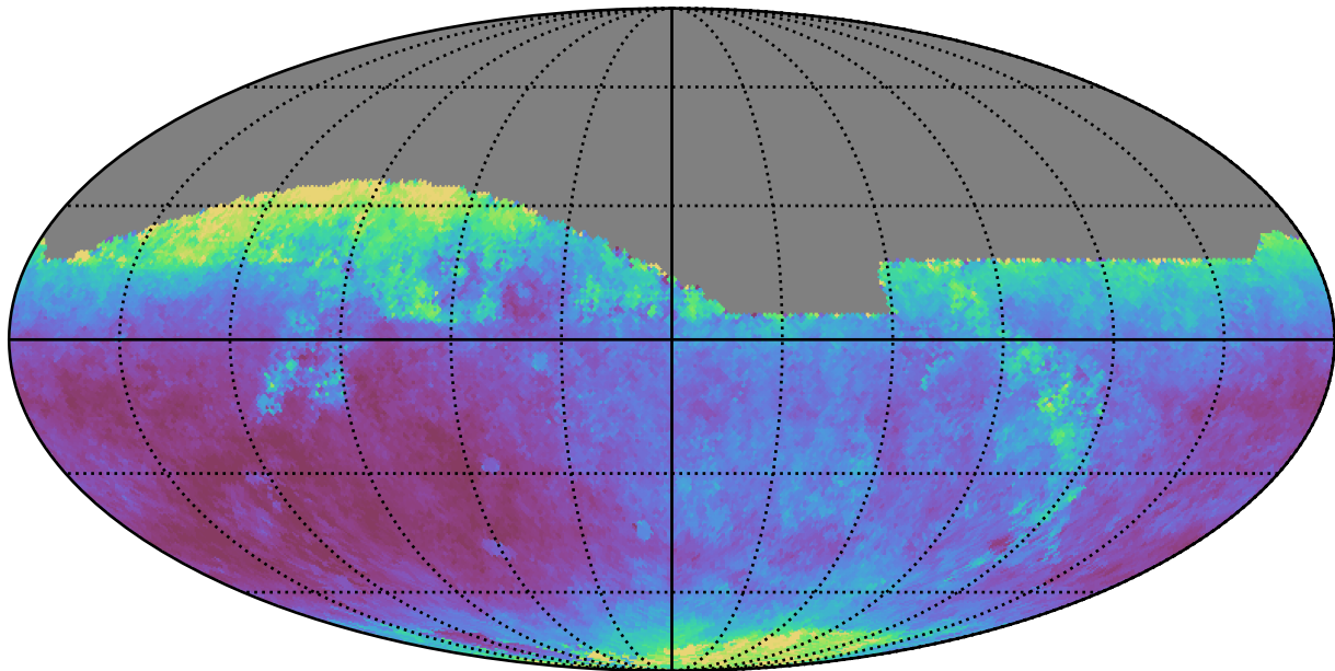
noroll_mjdp180_v3.4_10yrs All sky z band: Median seeingEff
