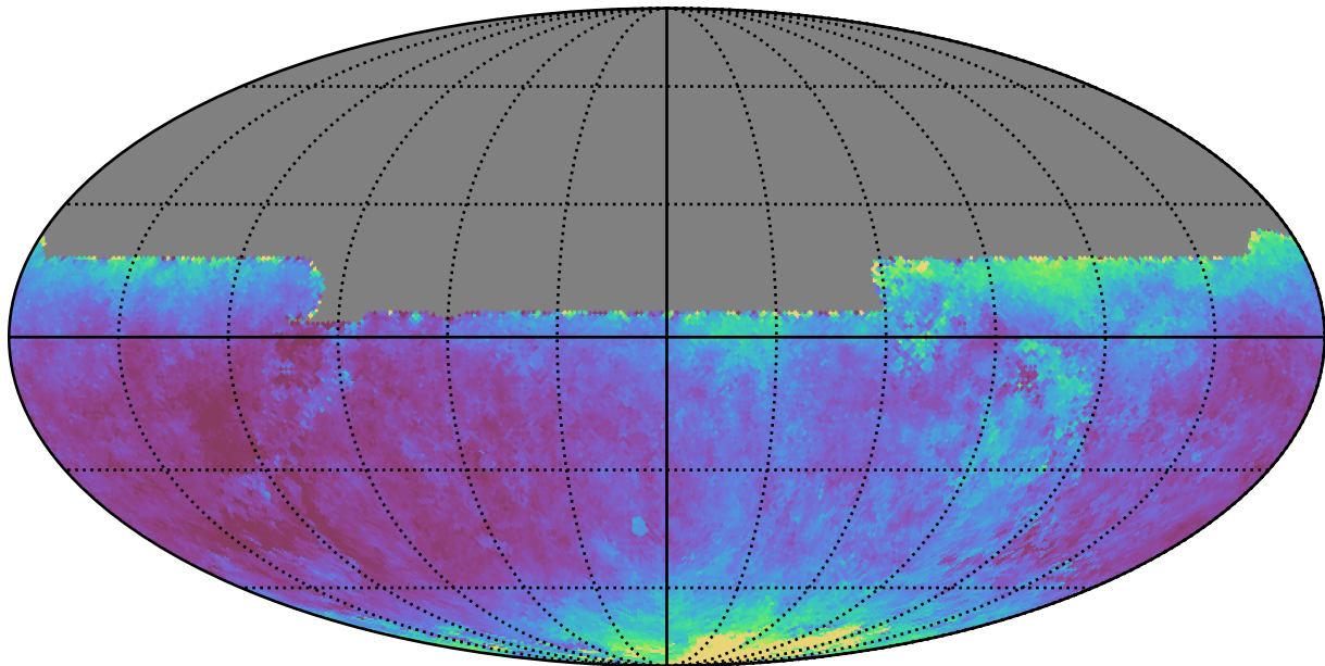
noroll_mjdp180_v3.4_10yrs All sky y band: Median seeingEff
