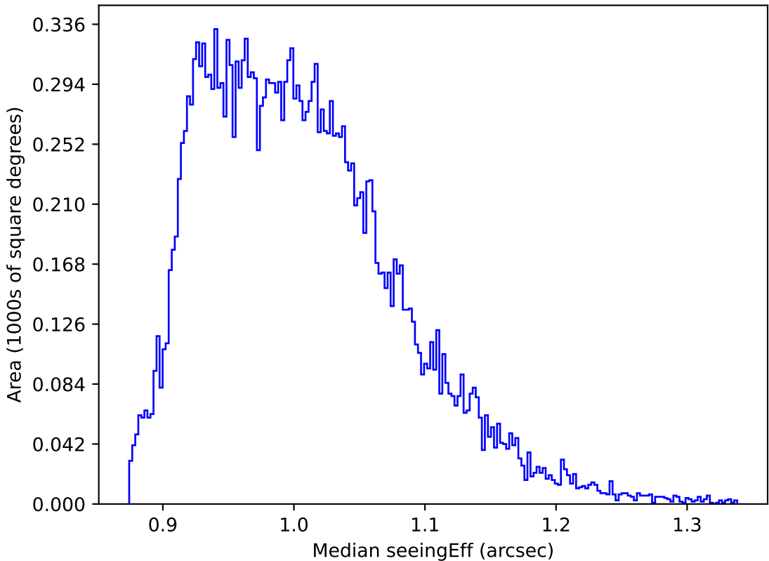
noroll_mjdp180_v3.4_10yrs All sky y band: Median seeingEff
