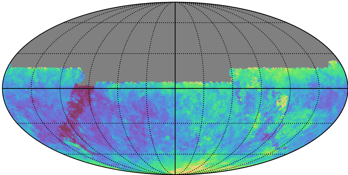
noroll_mjdp180_v3.4_10yrs All sky u band: Median seeingEff
