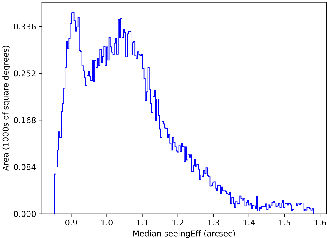
noroll_mjdp180_v3.4_10yrs All sky r band: Median seeingEff
