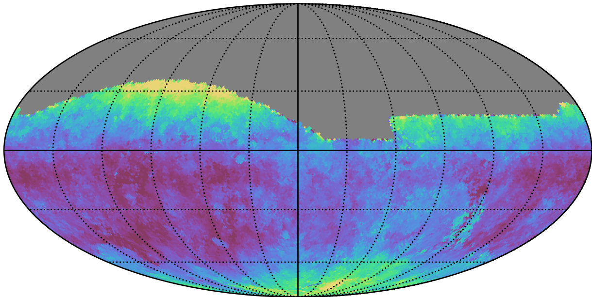
noroll_mjdp180_v3.4_10yrs All sky g band: Median seeingEff
