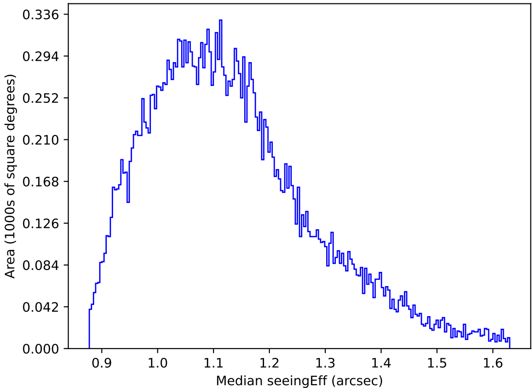
noroll_mjdp180_v3.4_10yrs All sky g band: Median seeingEff
