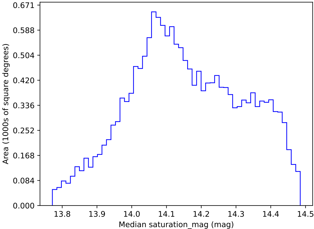
noroll_mjdp180_v3.4_10yrs WFD z band: Median saturation_mag
