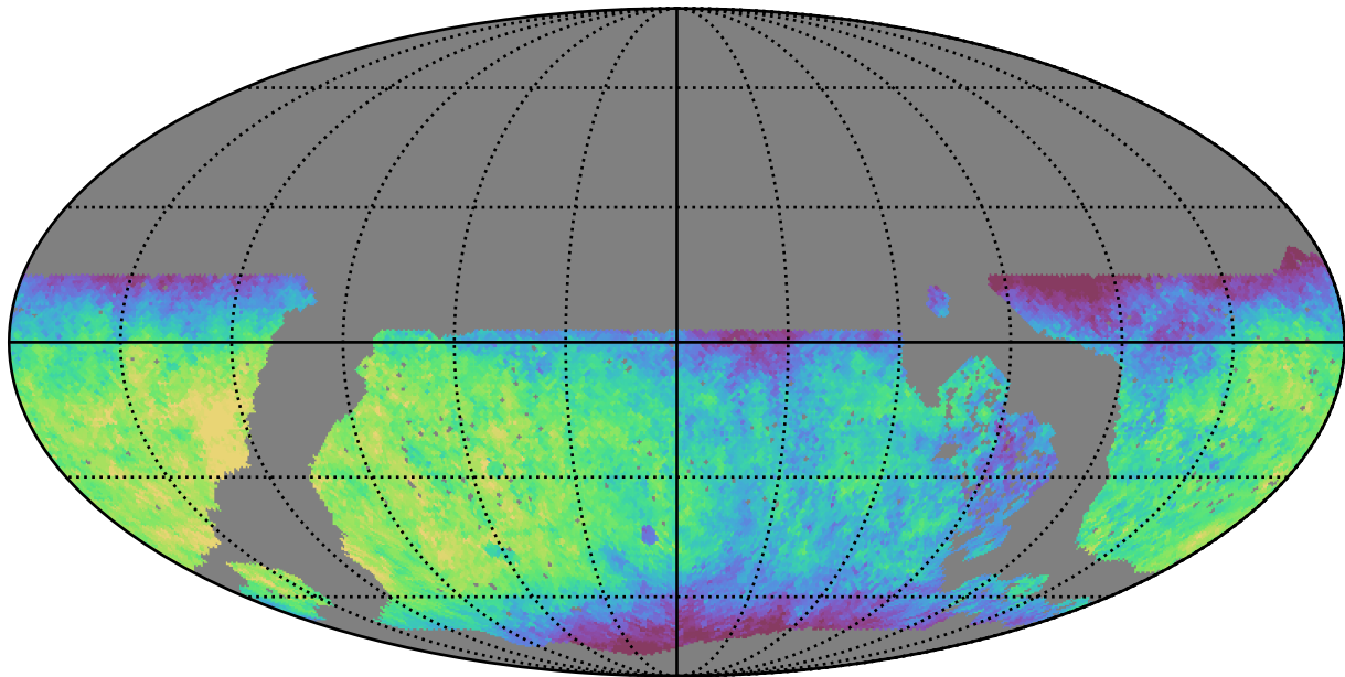
noroll_mjdp180_v3.4_10yrs WFD y band: Median saturation_mag
