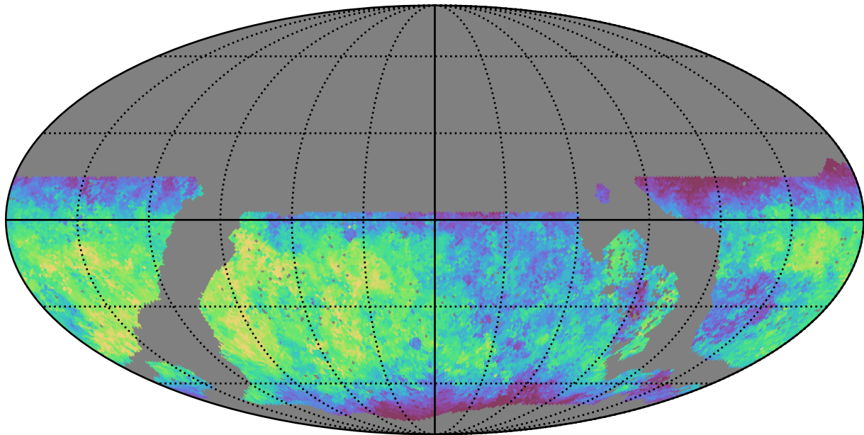
noroll_mjdp180_v3.4_10yrs WFD u band: Median saturation_mag
