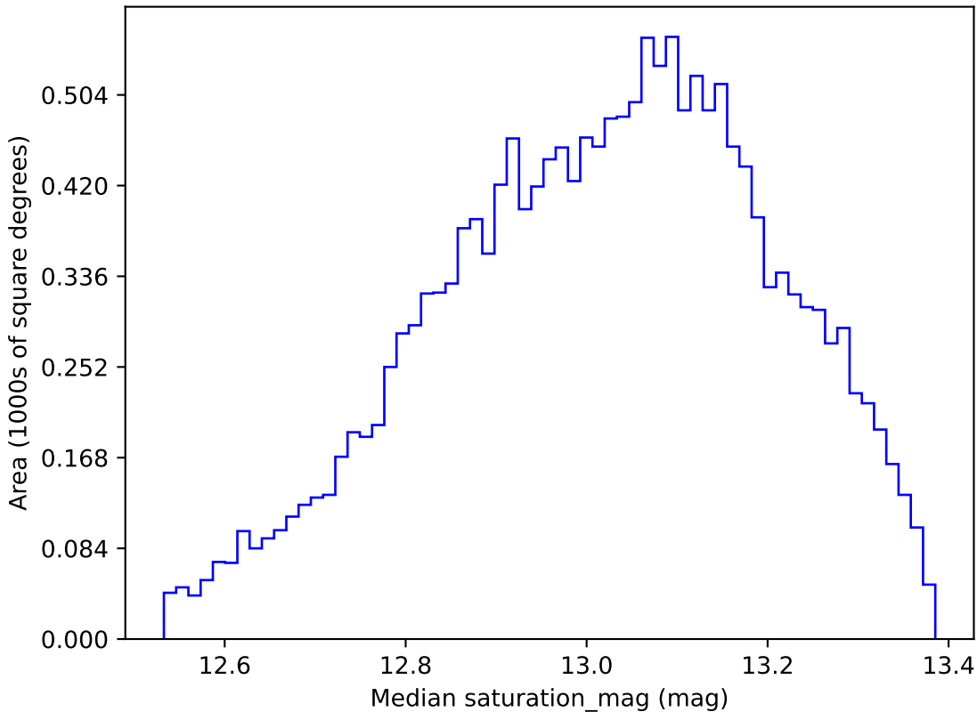
noroll_mjdp180_v3.4_10yrs WFD u band: Median saturation_mag
