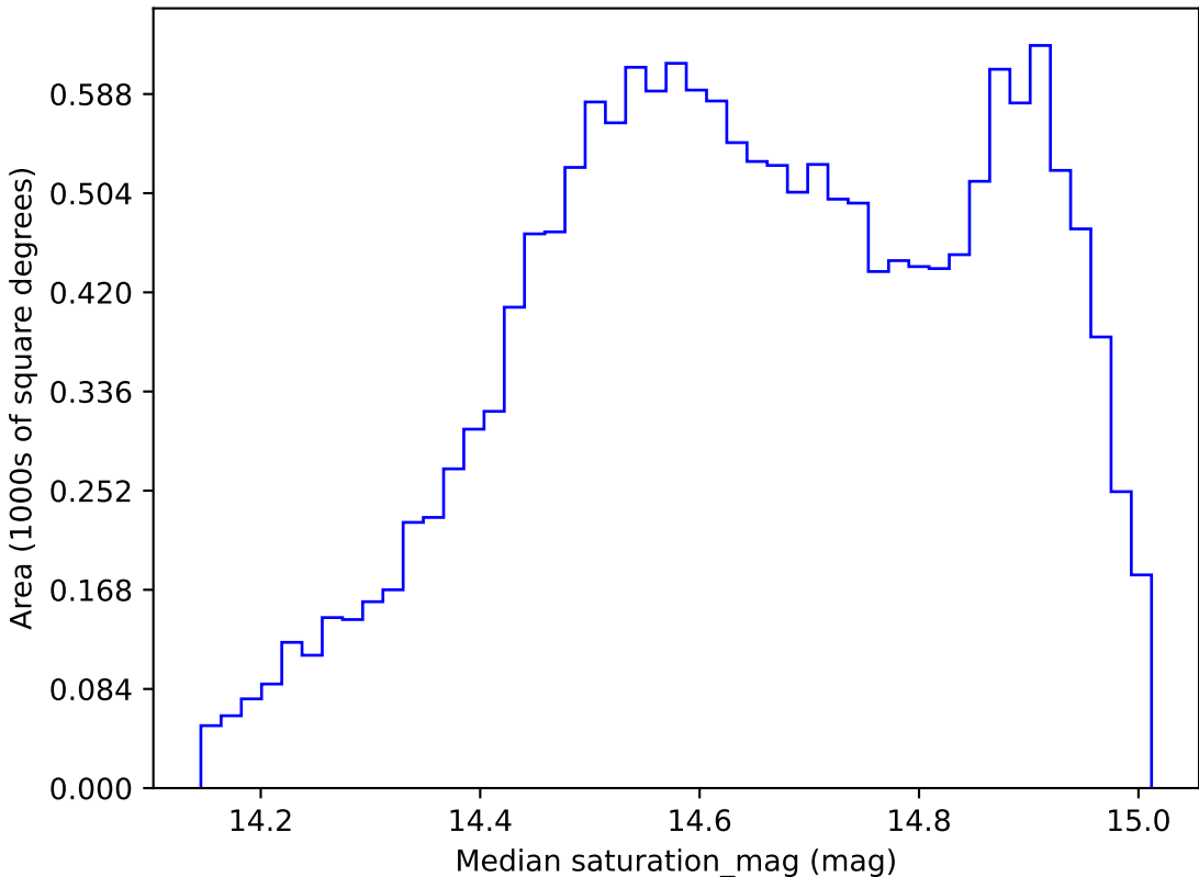
noroll_mjdp180_v3.4_10yrs WFD r band: Median saturation_mag
