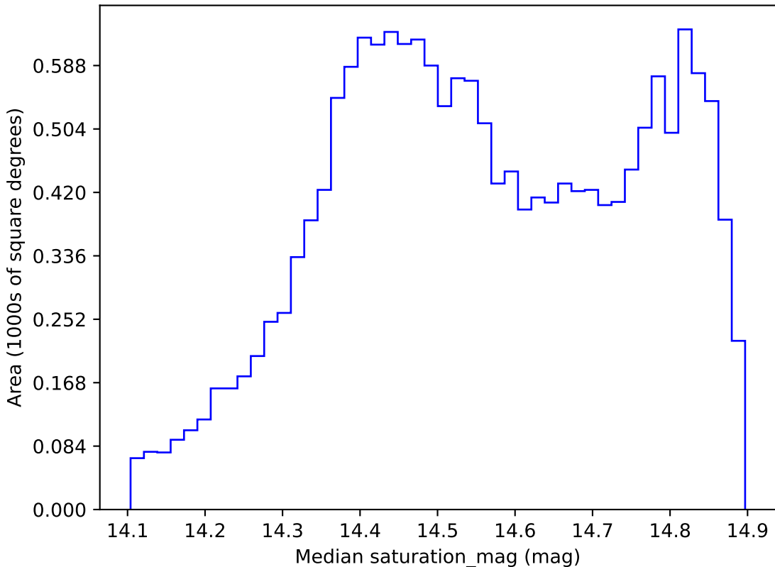
noroll_mjdp180_v3.4_10yrs WFD i band: Median saturation_mag
