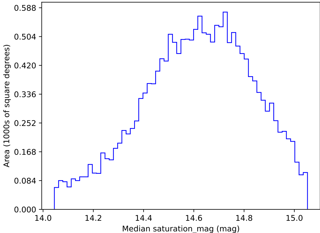
noroll_mjdp180_v3.4_10yrs WFD g band: Median saturation_mag
