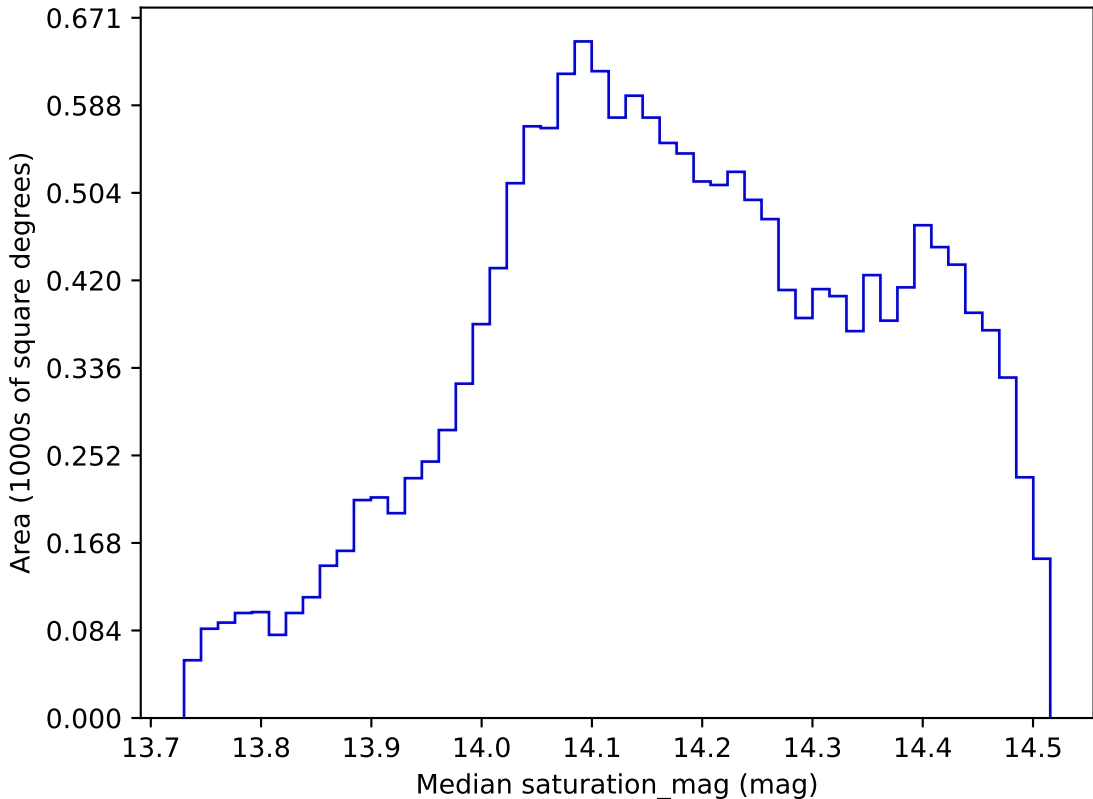
noroll_mjdp180_v3.4_10yrs WFD all bands: Median saturation_mag
