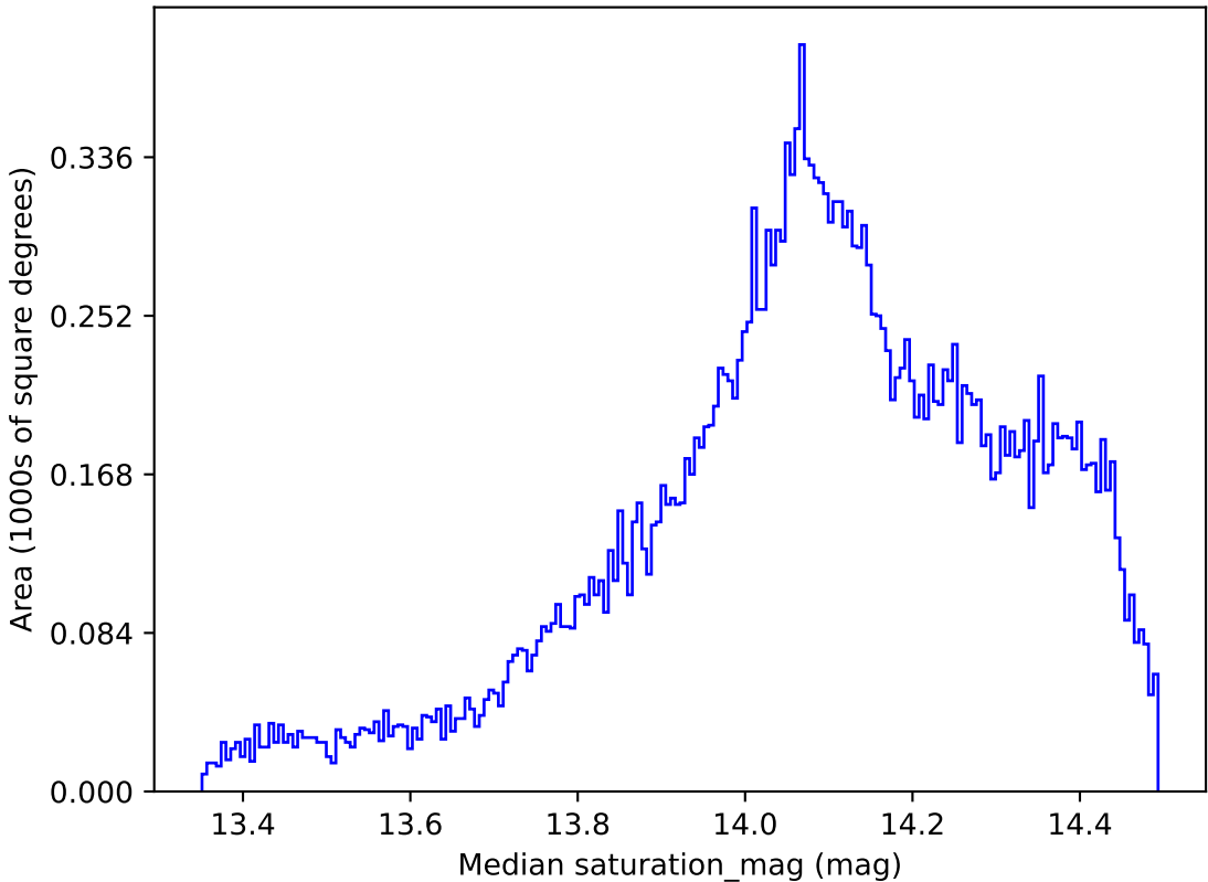
noroll_mjdp180_v3.4_10yrs All sky z band: Median saturation_mag
