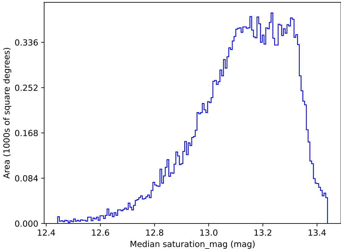
noroll_mjdp180_v3.4_10yrs All sky y band: Median saturation_mag
