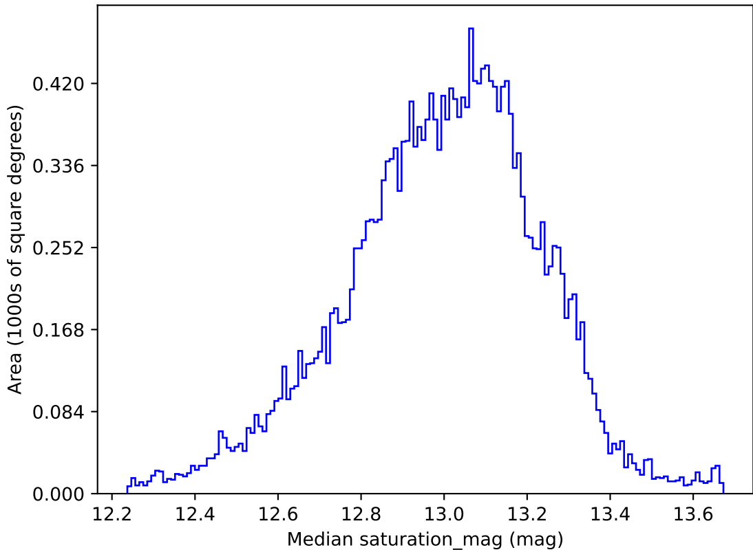
noroll_mjdp180_v3.4_10yrs All sky u band: Median saturation_mag
