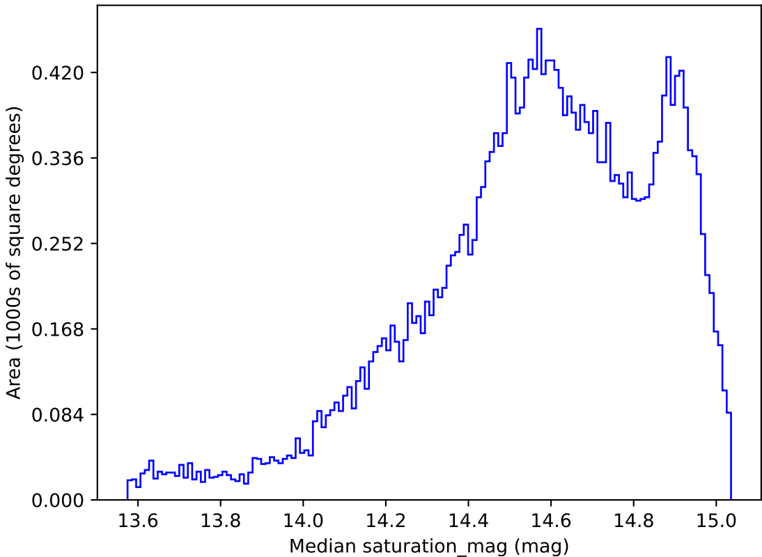
noroll_mjdp180_v3.4_10yrs All sky r band: Median saturation_mag
