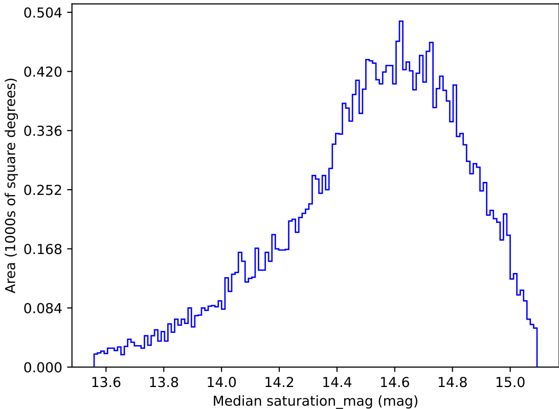
noroll_mjdp180_v3.4_10yrs All sky g band: Median saturation_mag
