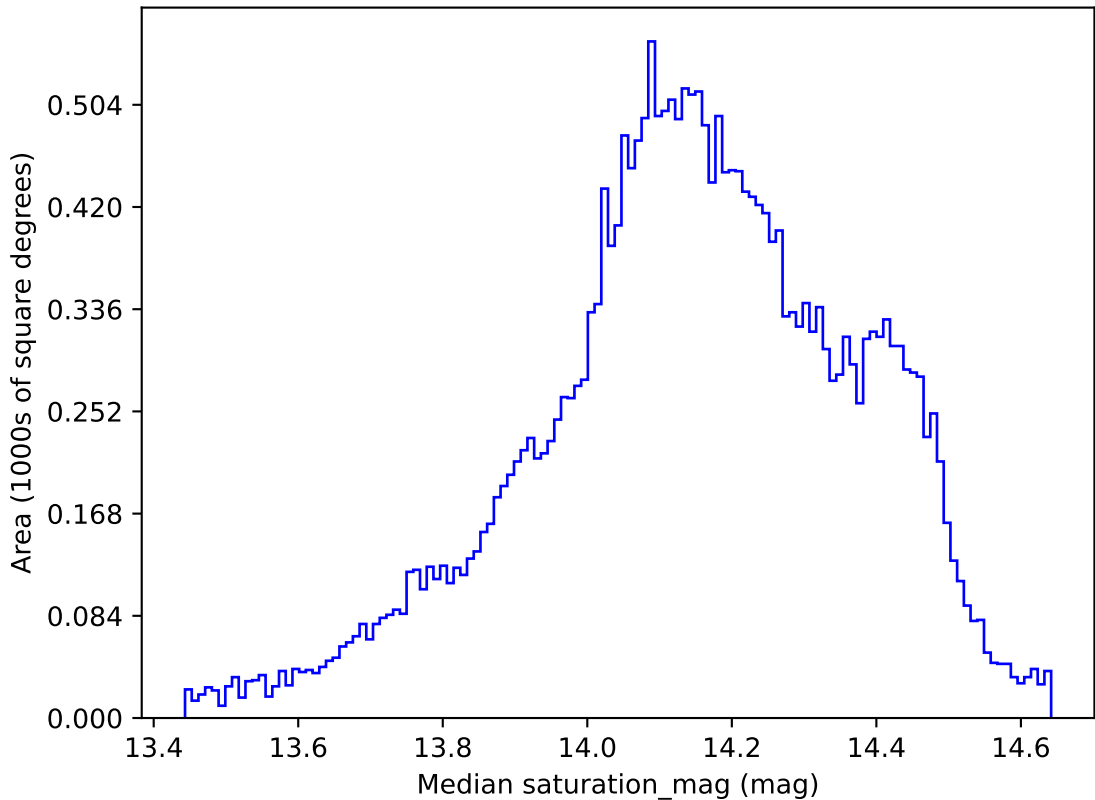
noroll_mjdp180_v3.4_10yrs All sky all bands: Median saturation_mag
