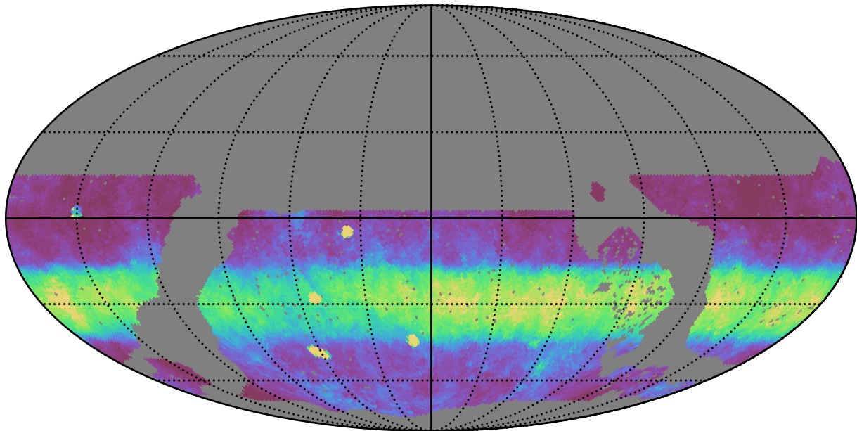
noroll_mjdp180_v3.4_10yrs WFD z band: Median normairmass
