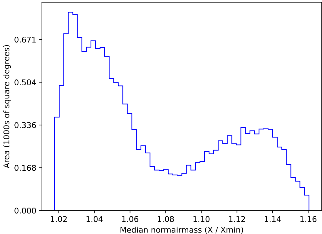
noroll_mjdp180_v3.4_10yrs WFD z band: Median normairmass
