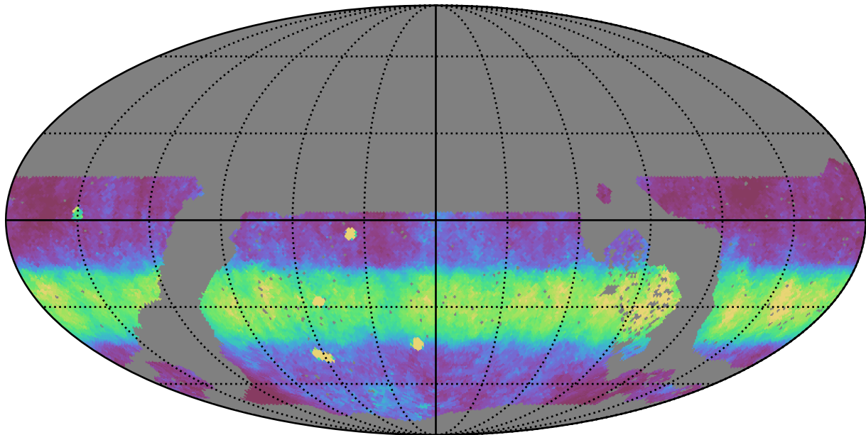
noroll_mjdp180_v3.4_10yrs WFD y band: Median normairmass
