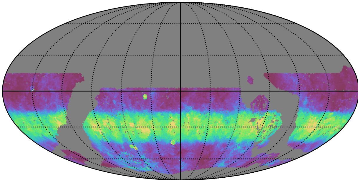
noroll_mjdp180_v3.4_10yrs WFD u band: Median normairmass
