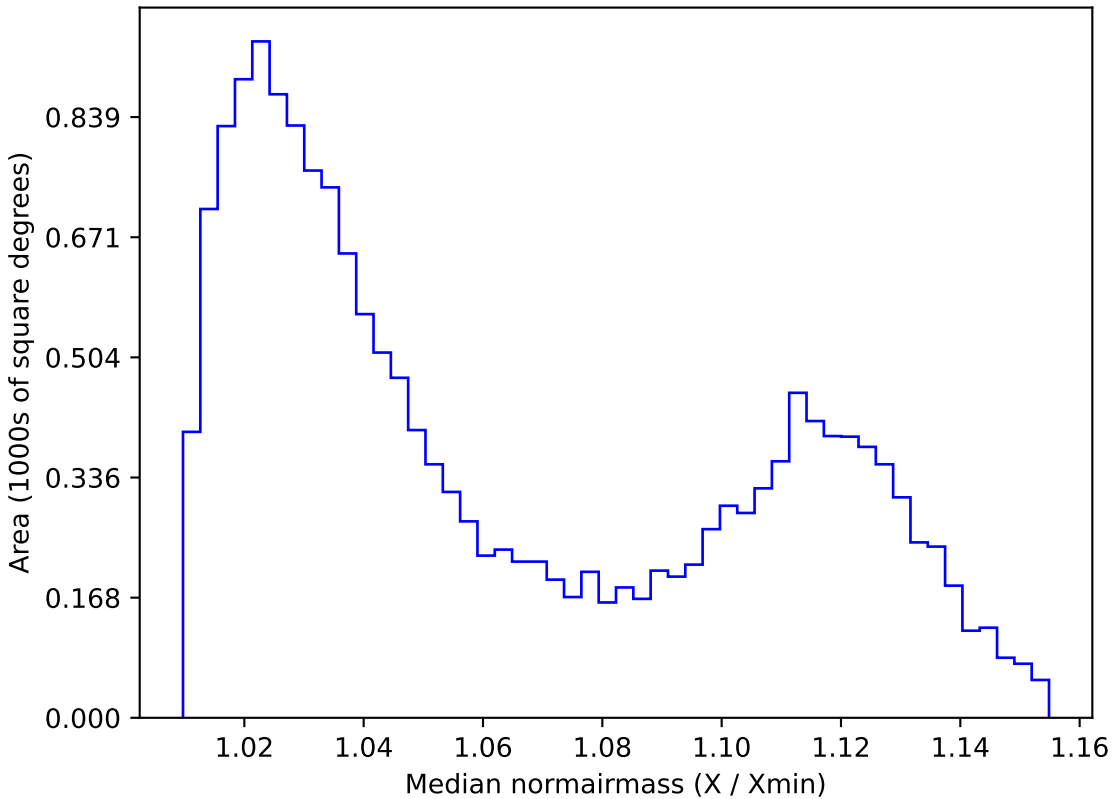
noroll_mjdp180_v3.4_10yrs WFD u band: Median normairmass
