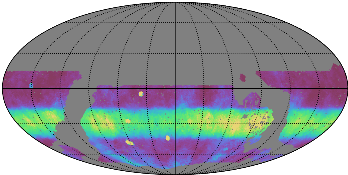
noroll_mjdp180_v3.4_10yrs WFD r band: Median normairmass
