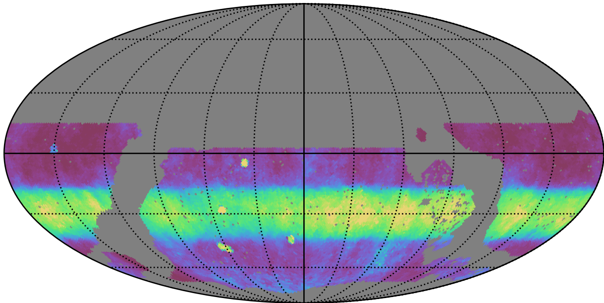
noroll_mjdp180_v3.4_10yrs WFD i band: Median normairmass
