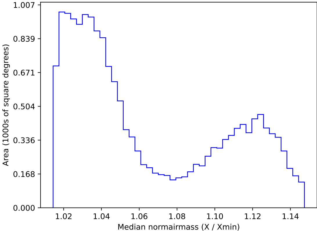
noroll_mjdp180_v3.4_10yrs WFD i band: Median normairmass
