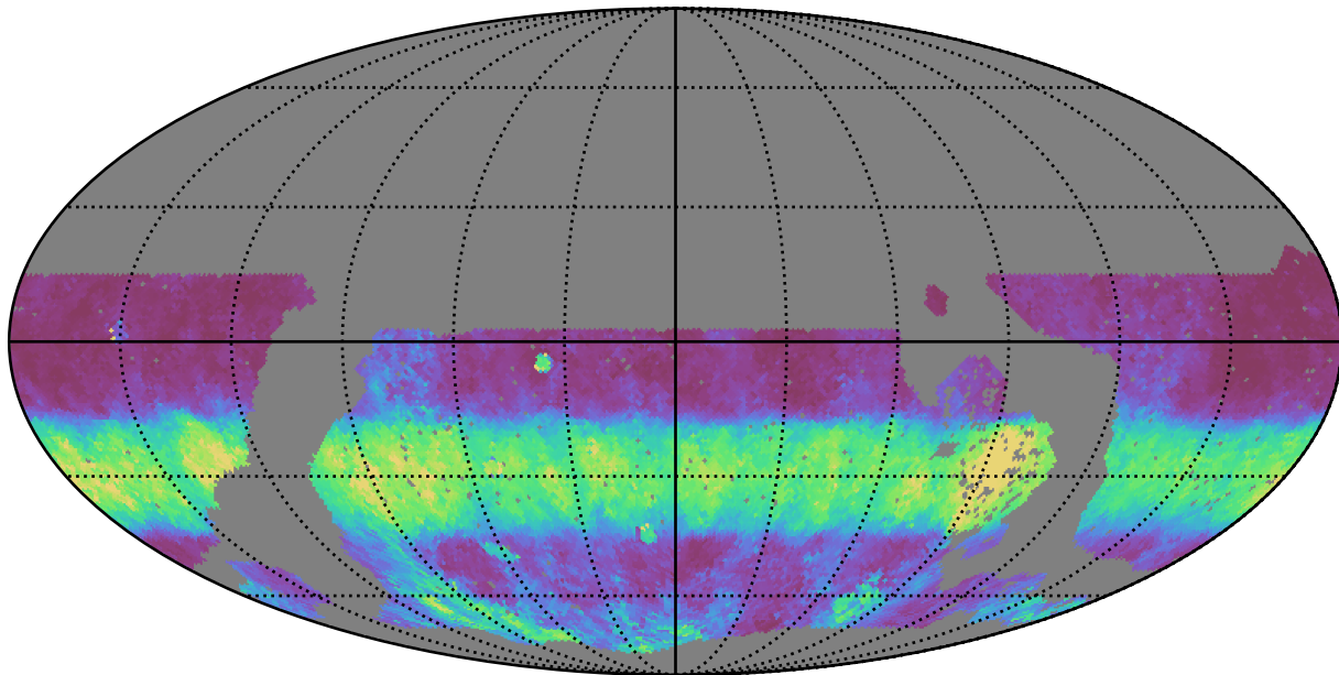
noroll_mjdp180_v3.4_10yrs WFD g band: Median normairmass
