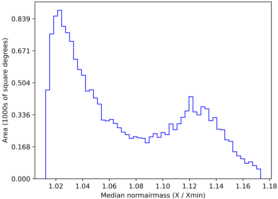
noroll_mjdp180_v3.4_10yrs WFD g band: Median normairmass
