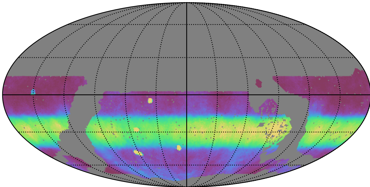
noroll_mjdp180_v3.4_10yrs WFD all bands: Median normairmass
