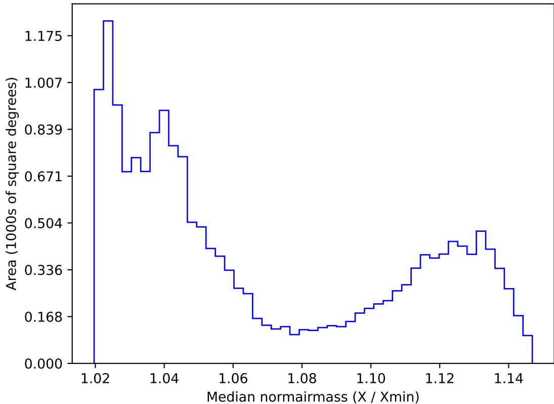
noroll_mjdp180_v3.4_10yrs WFD all bands: Median normairmass
