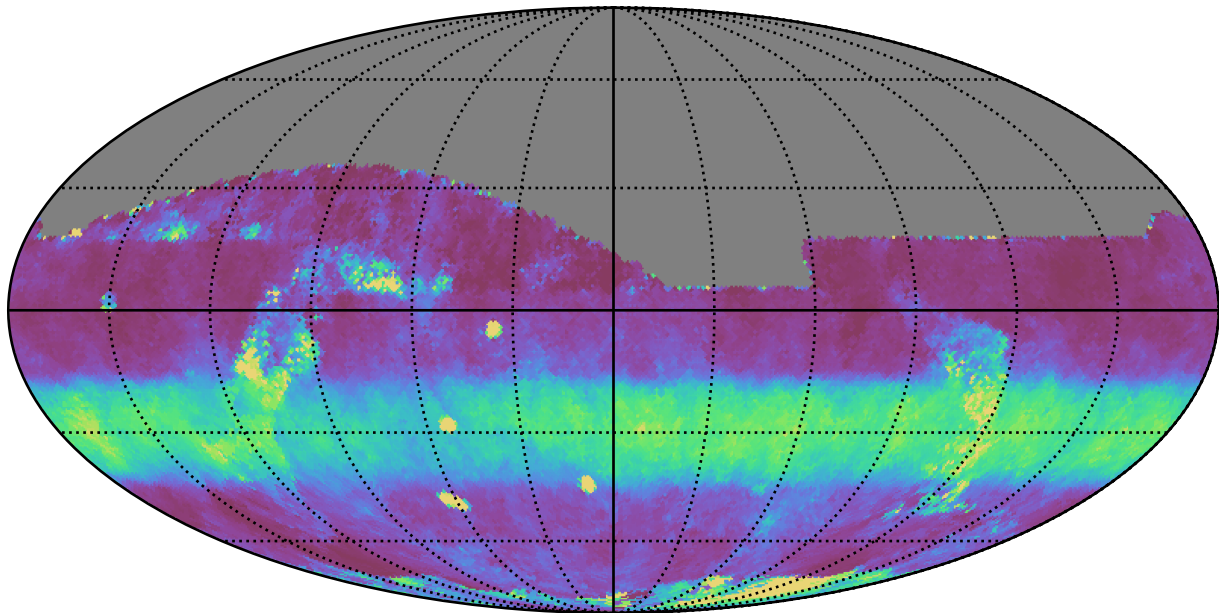
noroll_mjdp180_v3.4_10yrs All sky z band: Median normairmass
