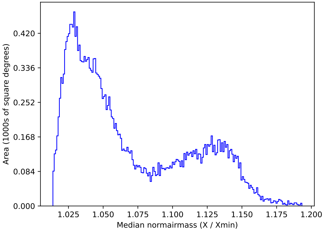
noroll_mjdp180_v3.4_10yrs All sky z band: Median normairmass
