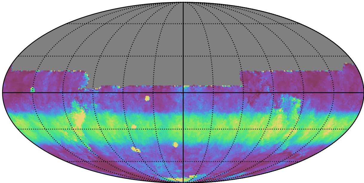
noroll_mjdp180_v3.4_10yrs All sky y band: Median normairmass
