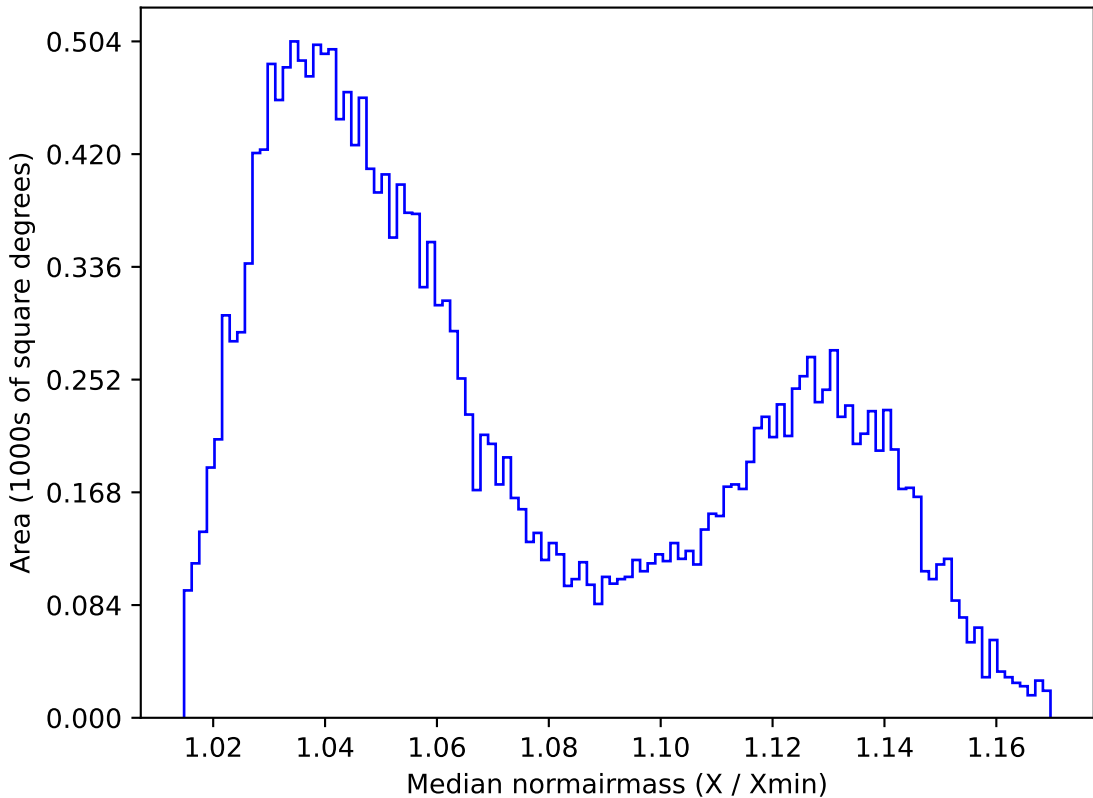
noroll_mjdp180_v3.4_10yrs All sky y band: Median normairmass
