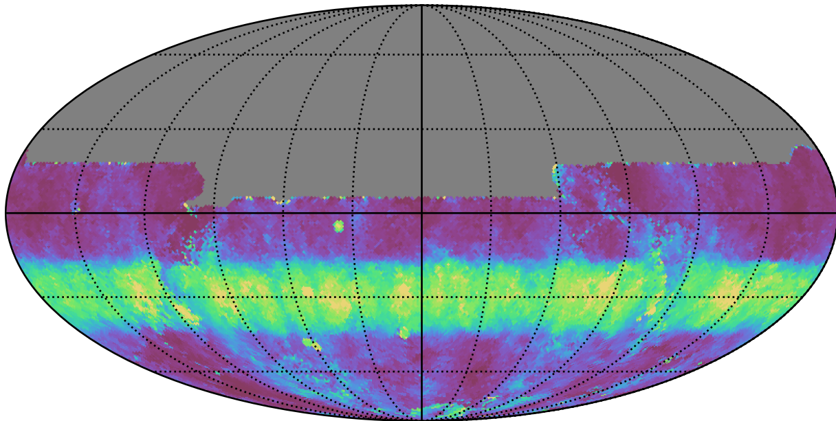
noroll_mjdp180_v3.4_10yrs All sky u band: Median normairmass
