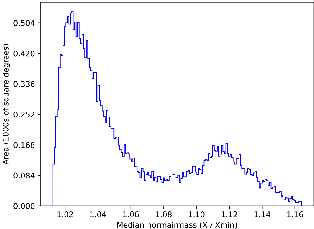
noroll_mjdp180_v3.4_10yrs All sky r band: Median normairmass
