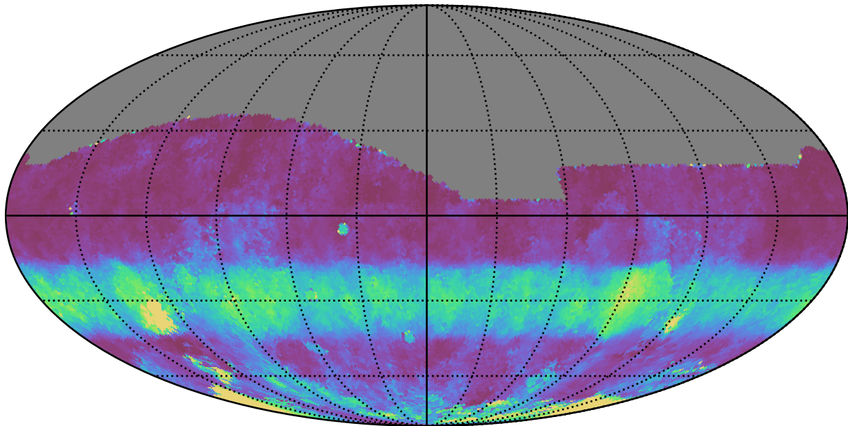
noroll_mjdp180_v3.4_10yrs All sky g band: Median normairmass
