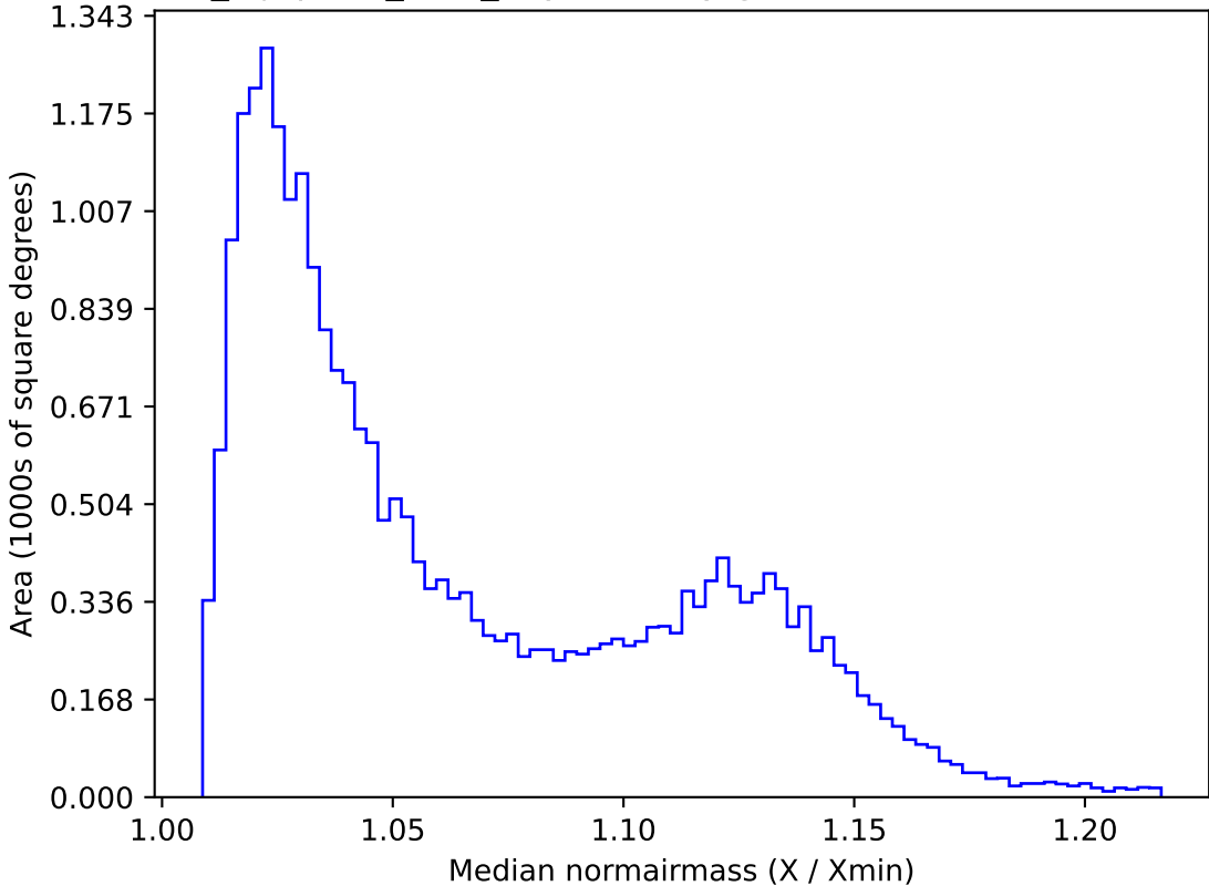
noroll_mjdp180_v3.4_10yrs All sky g band: Median normairmass
