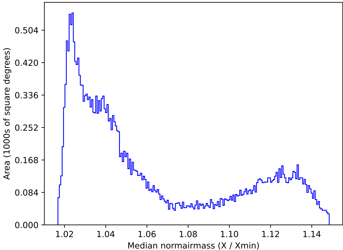
noroll_mjdp180_v3.4_10yrs All sky all bands: Median normairmass
