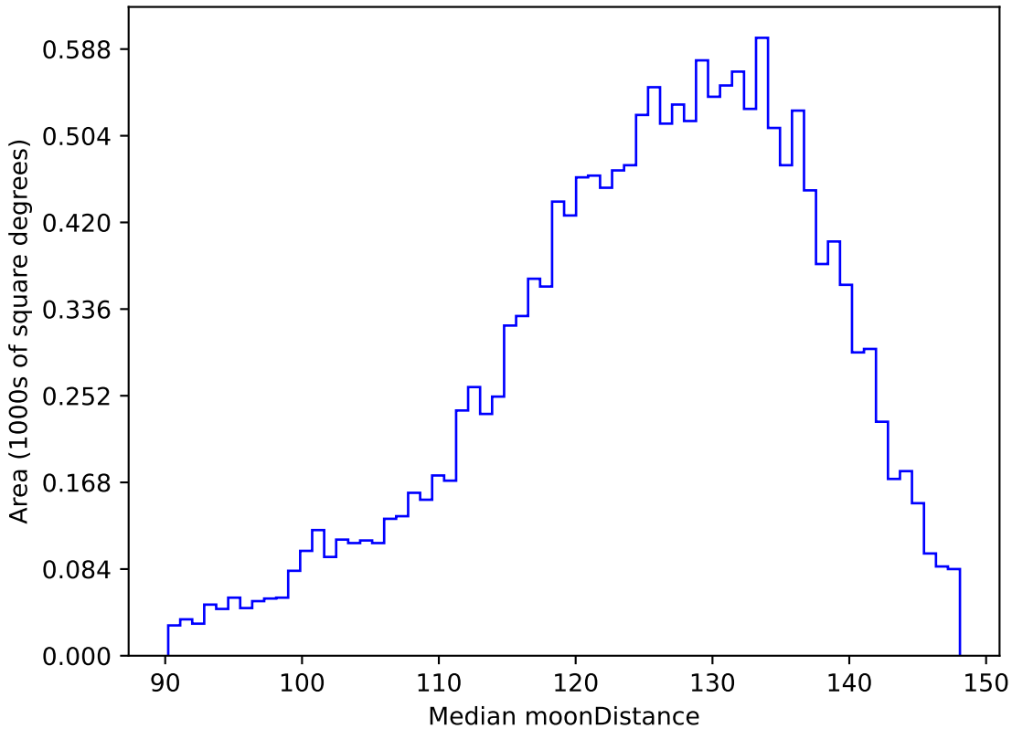
noroll_mjdp180_v3.4_10yrs WFD u band: Median moonDistance
