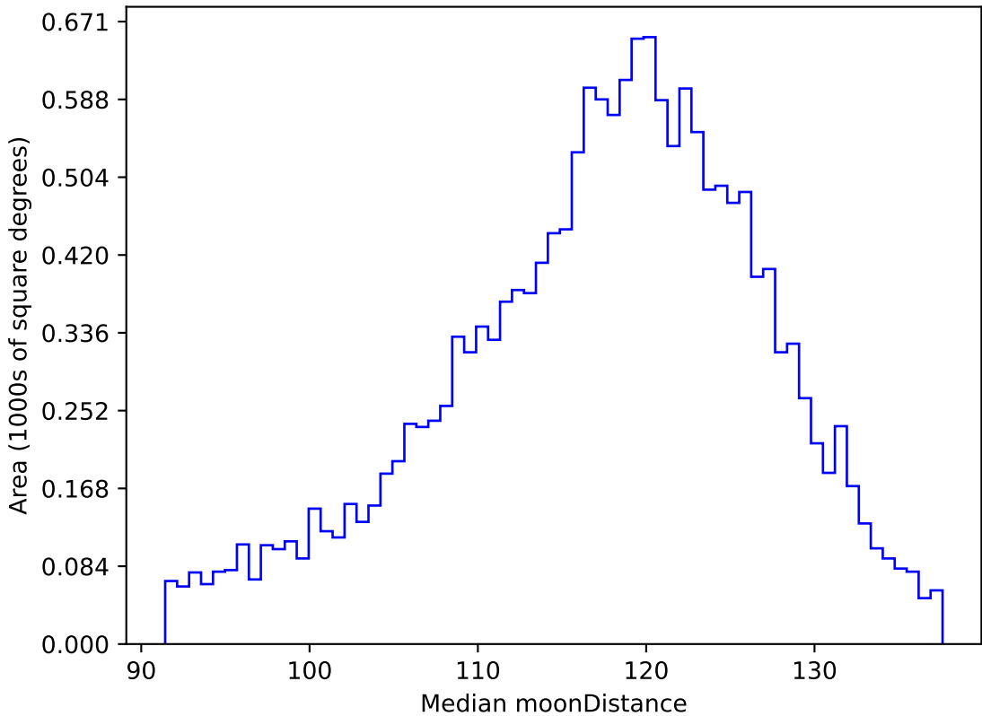
noroll_mjdp180_v3.4_10yrs WFD g band: Median moonDistance
