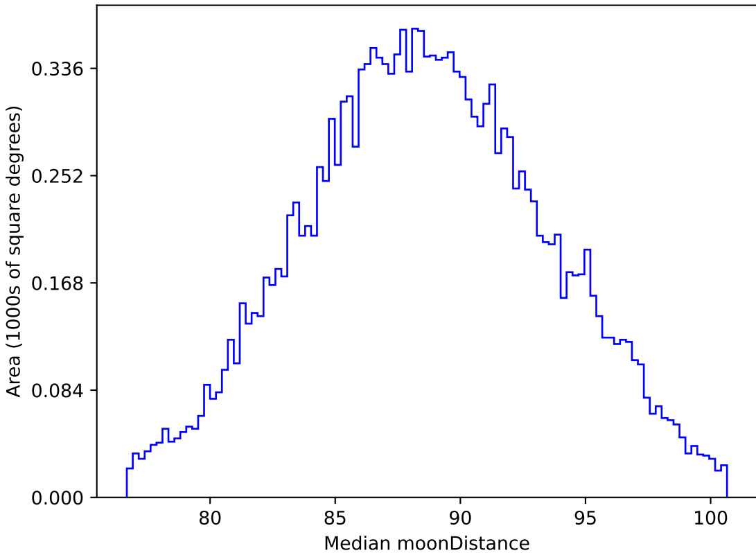
noroll_mjdp180_v3.4_10yrs WFD all bands: Median moonDistance
